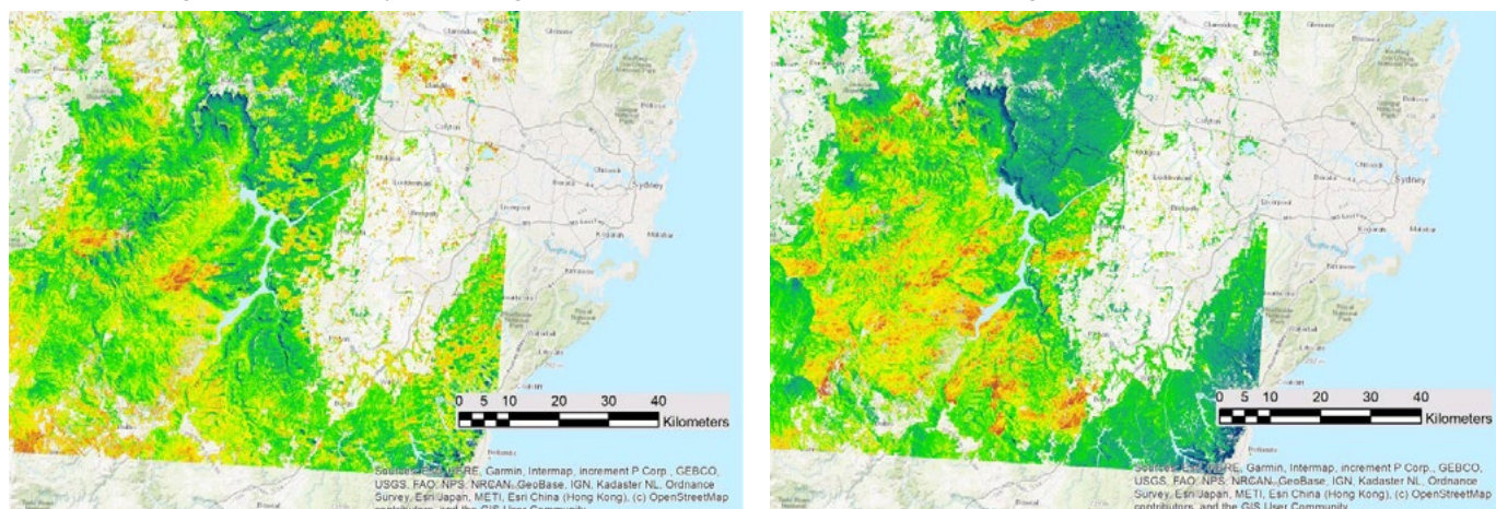
Figure 2. Maps showing the differences in spatial extent and variability of the bushfires in New South Wales between the 1st and 31st of December. Green means mostly untouched vegetation; the redder the colour, the higher the impact on the forests. Source: bit.ly/2VOPlcB
